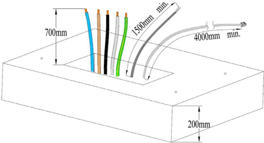
Figure 3.2-B Base and cable reservation requirements
