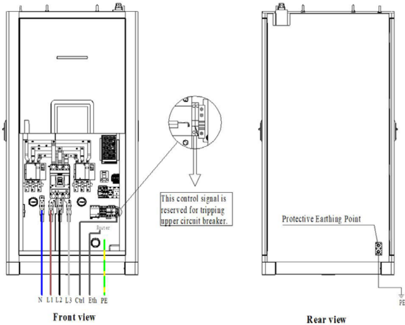
Figure 3.4-A Internal wiring diagram of charger
