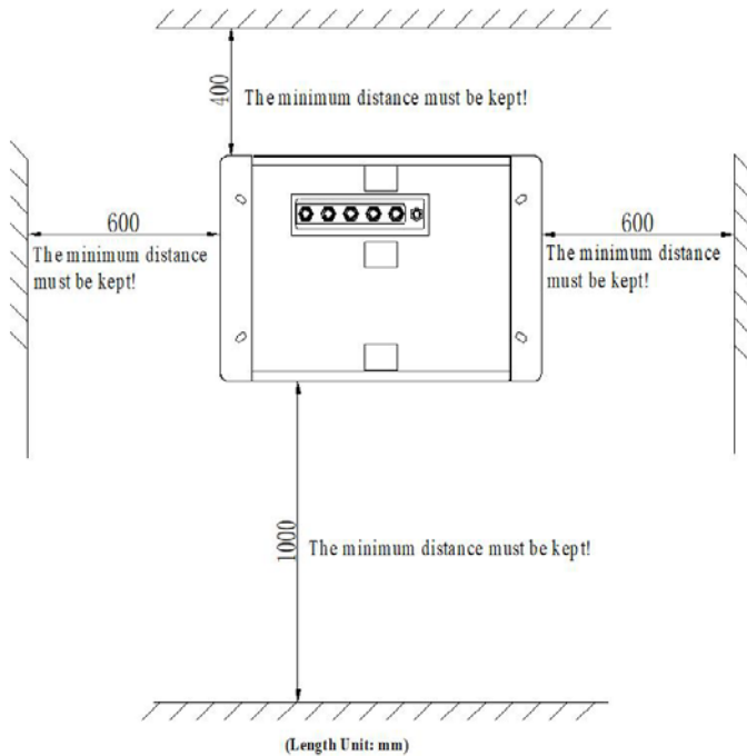
Figure 3.2-A Requirements for charger placement
