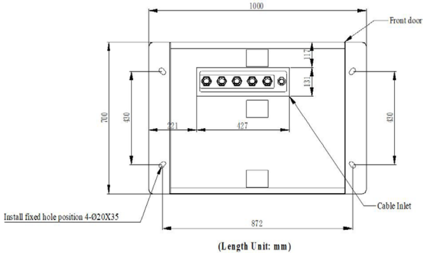
Figure 3.1-B Hole size of charger base
