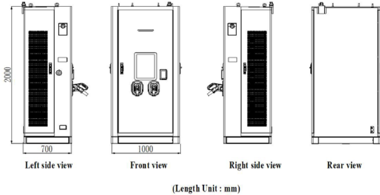
Figure 3.1-A Outline and dimension of charger
