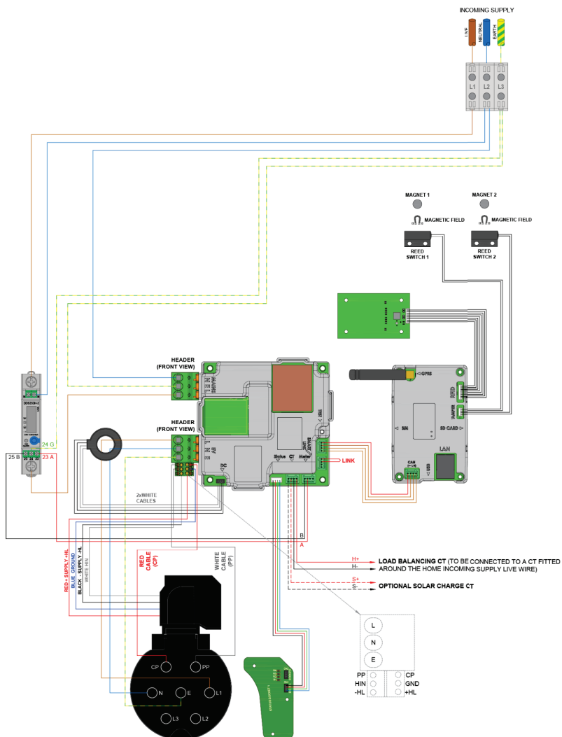
Figure 24 Zura Intelligent EV Charging Unit (Single-Phase) – 1x up to 7.4kW Type 2 Socket
