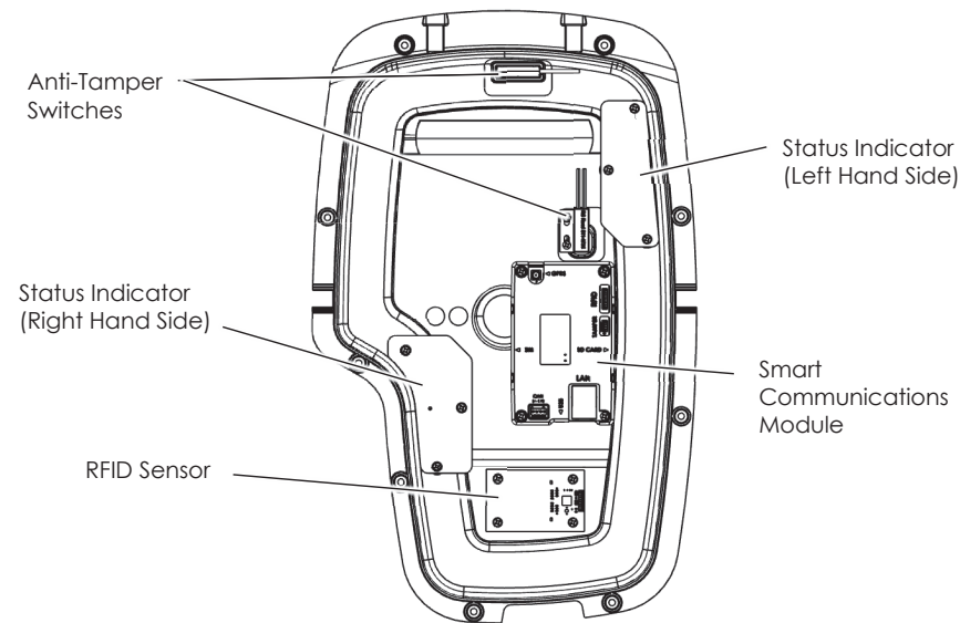
Figure 11 Zura Protective Components
