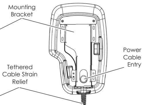
Figure 9 Zura 2 x Tethered Chargepoint (Rear)
