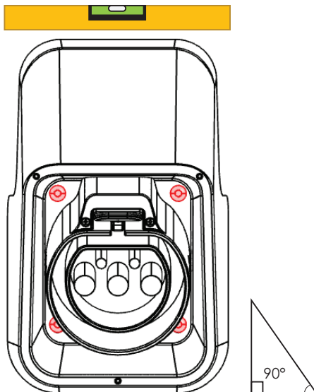
Figure 40 Mount the Plug Holster
