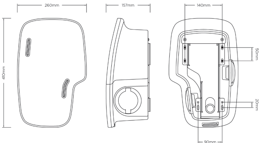
Figure 14 Zura Dimensions
