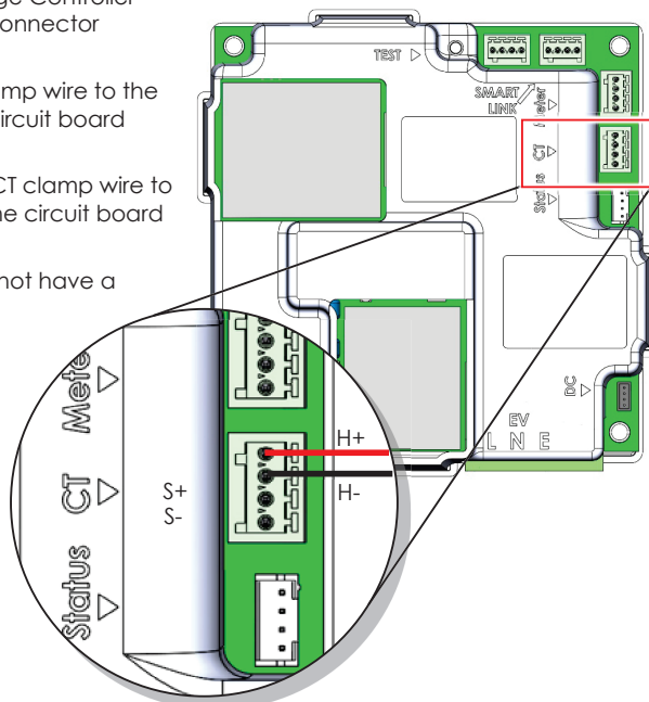
Figure 37 1-PH Load Balancing CT Connection
