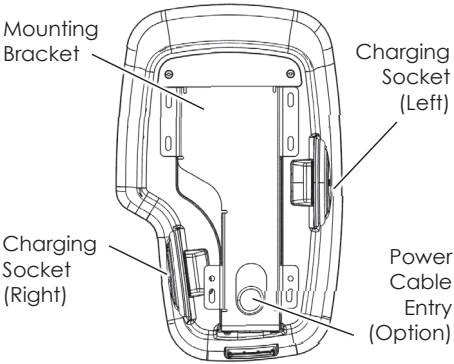
Figure 2 Zura 2 x Socket Chargepoint (Rear)
