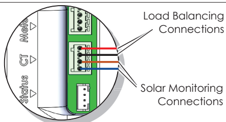
Figure 38 CT Connections for Load Balancing and Solar Monitoring
