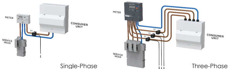
Figure 14 CT Clamp Positioning
