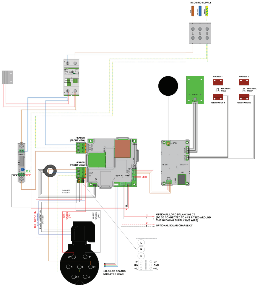
Figure 10 SecuriCharge Intelligent EV Charging Unit (Single-Phase) – 1x up to 7.4kW Type 2 Socket
