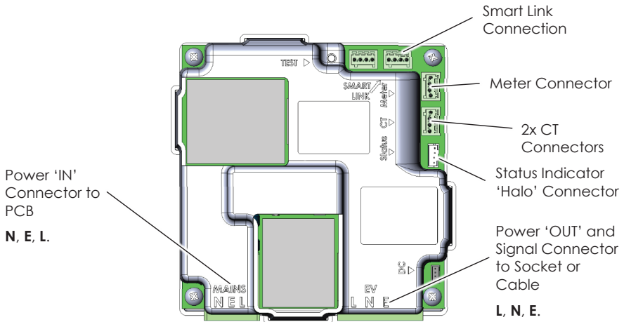
Figure 3 EV Charge Controller
