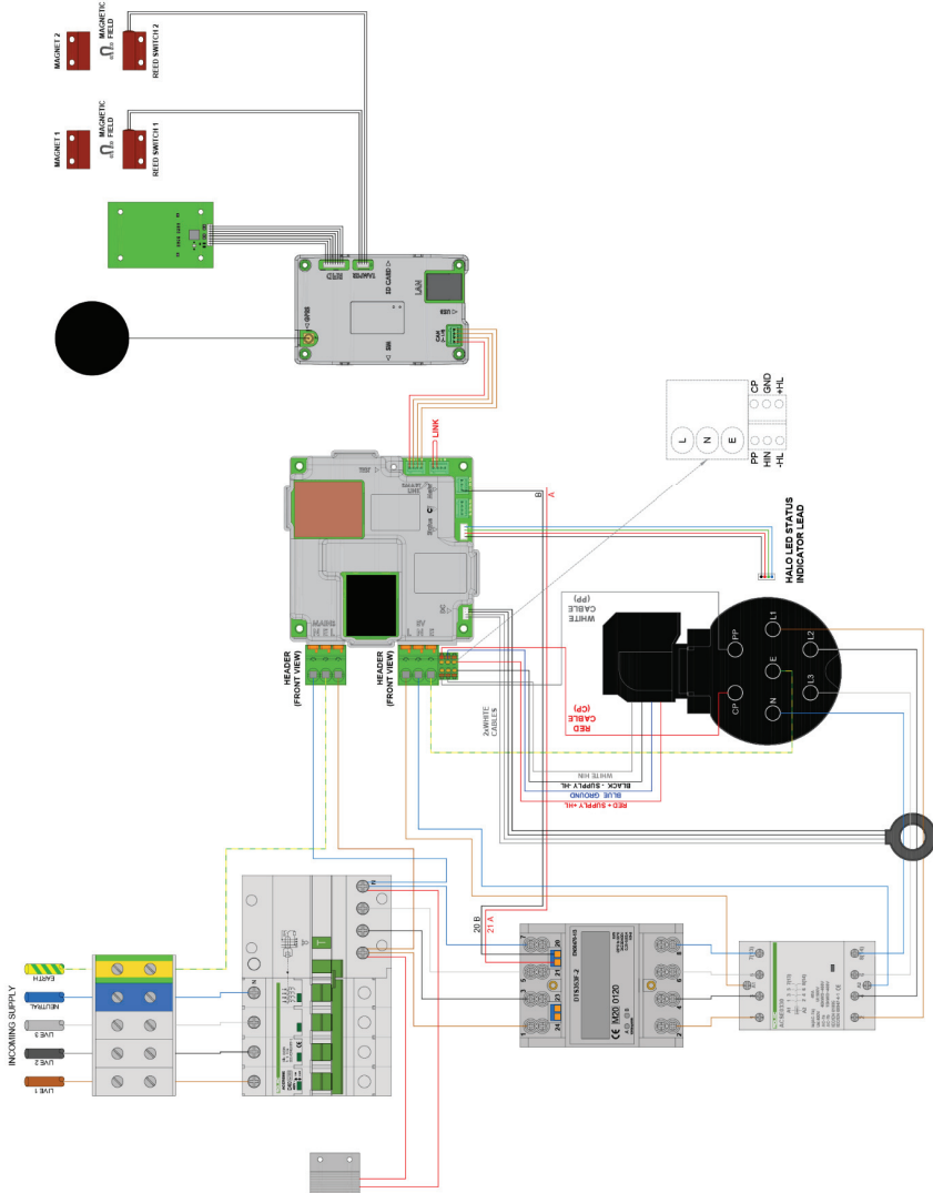
Figure 12 SecuriCharge Intelligent EV Charging Unit (Three-Phase) – 1x up to 22kW Type 2 Socket
