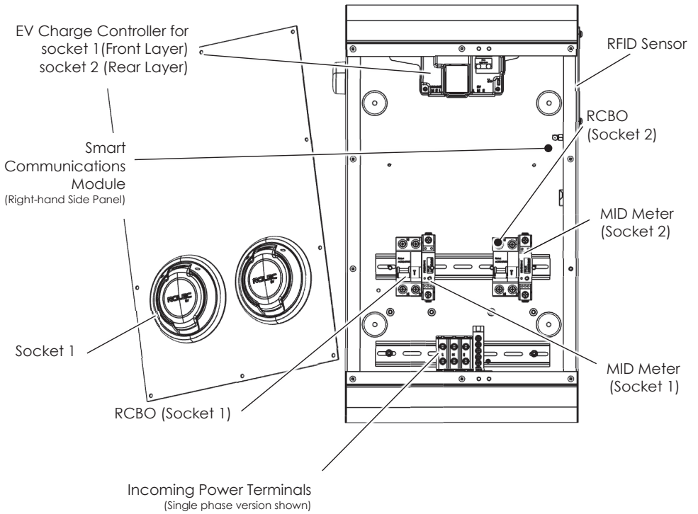
Figure 2 Internal Components - Typical Locations
