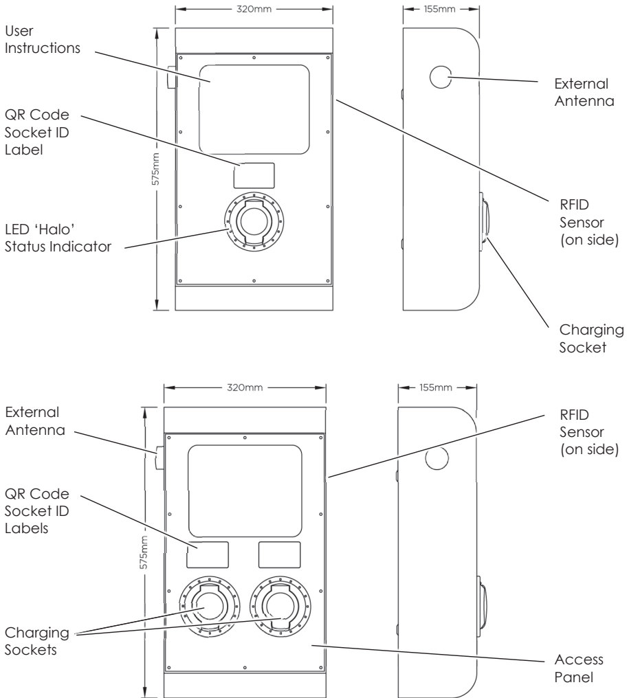
Figure 1 General Arrangement and Dimensions (Single and Double Socket Models)
