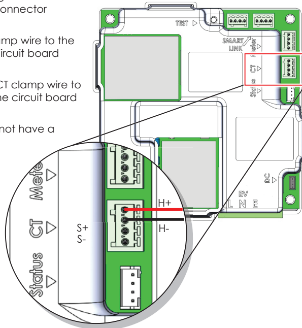
Figure 15 Load Balancing CT Connection
