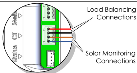
Figure 15 CT Connections for Load Balancing and Solar Monitoring
