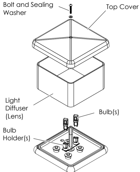
Figure 16 Lighting Head
