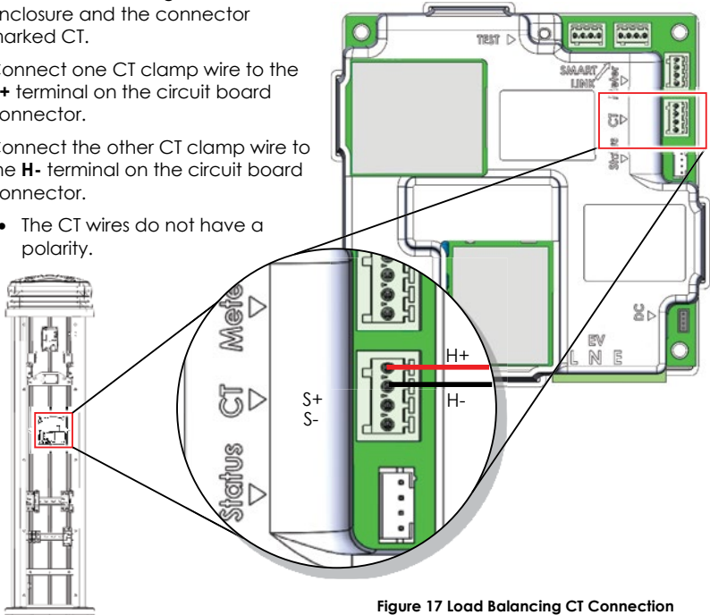
Figure 17 Load Balancing CT Connection
