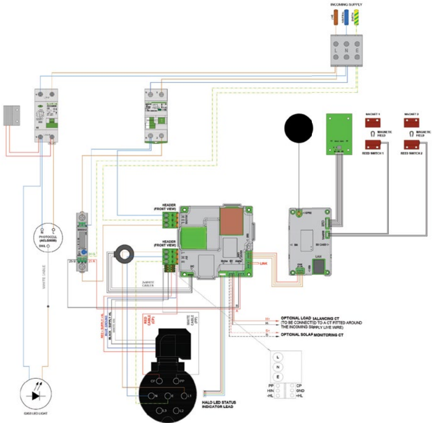
Figure 11 Quantum Intelligent EV Charging Pedestal (Single-Phase) – 1x up to 7.4kW Type 2 Socket
