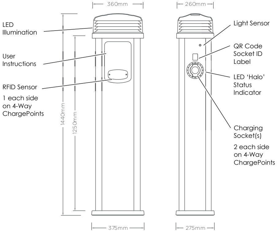
Figure 1 Pedestal General Arrangement and Dimensions
