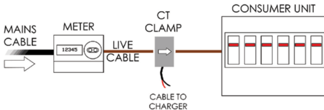
Figure 16 CT Clamp Positioning
