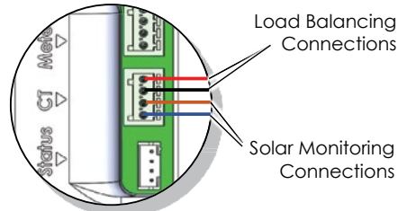
Figure 18 CT Connections for Load Balancing and Solar Monitoring
