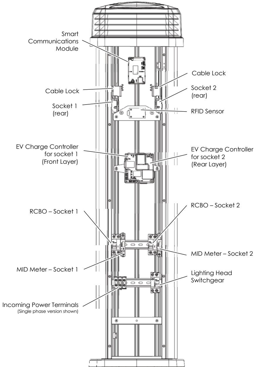
Figure 3 Internal Components - Typical Locations
