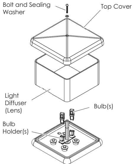
Figure 10 Lighting Head
