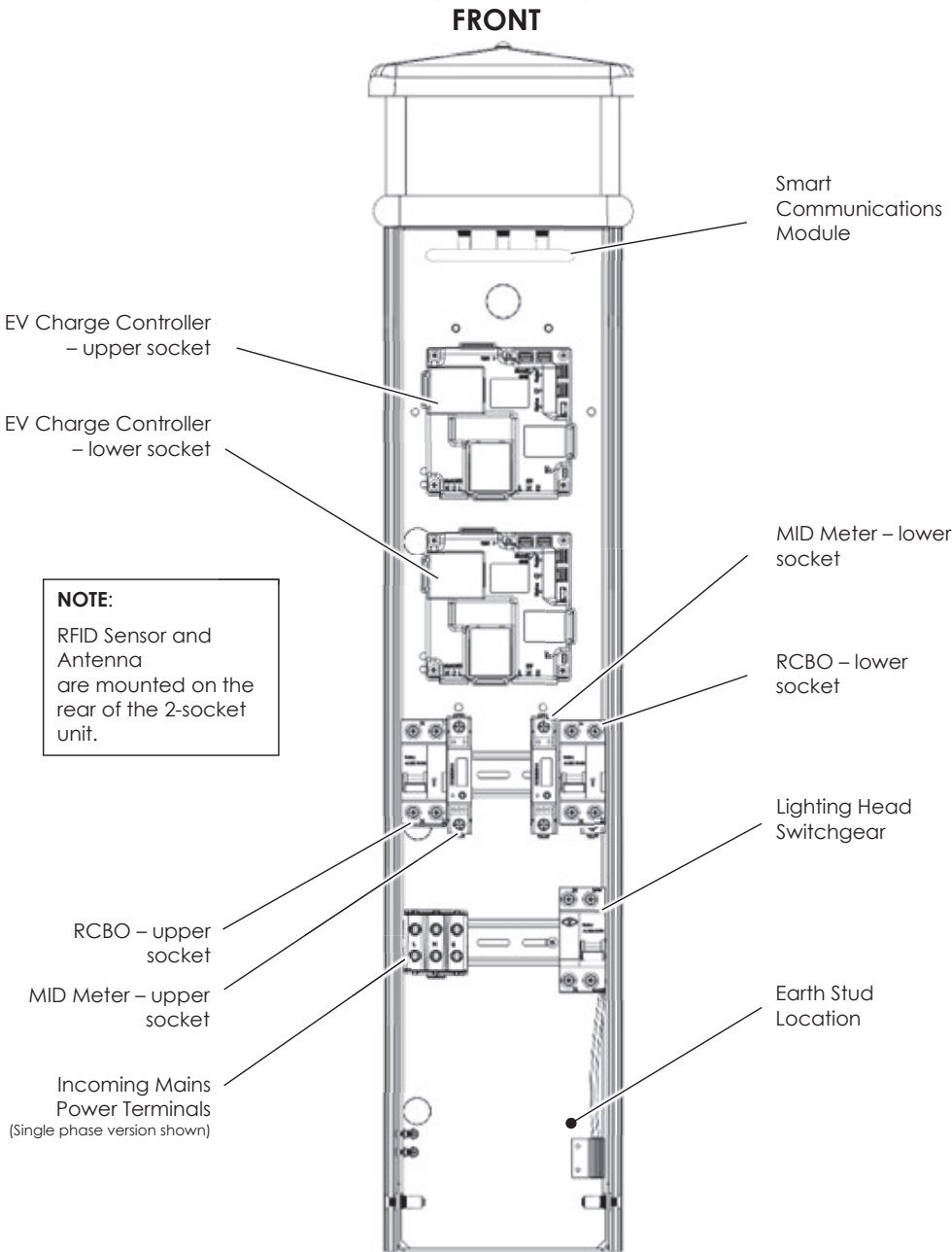
Figure 3 Internal Components - Typical Locations
