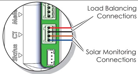
Figure 9 CT Connections for Load Balancing and Solar Monitoring
