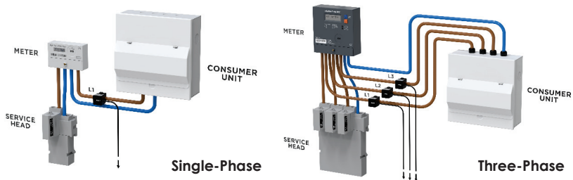
Figure 7 CT Clamp Positioning
