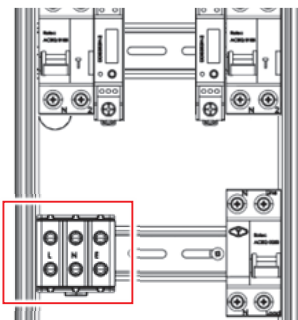
Figure 6 Incoming Mains Power Terminals (Single Phase Shown)
