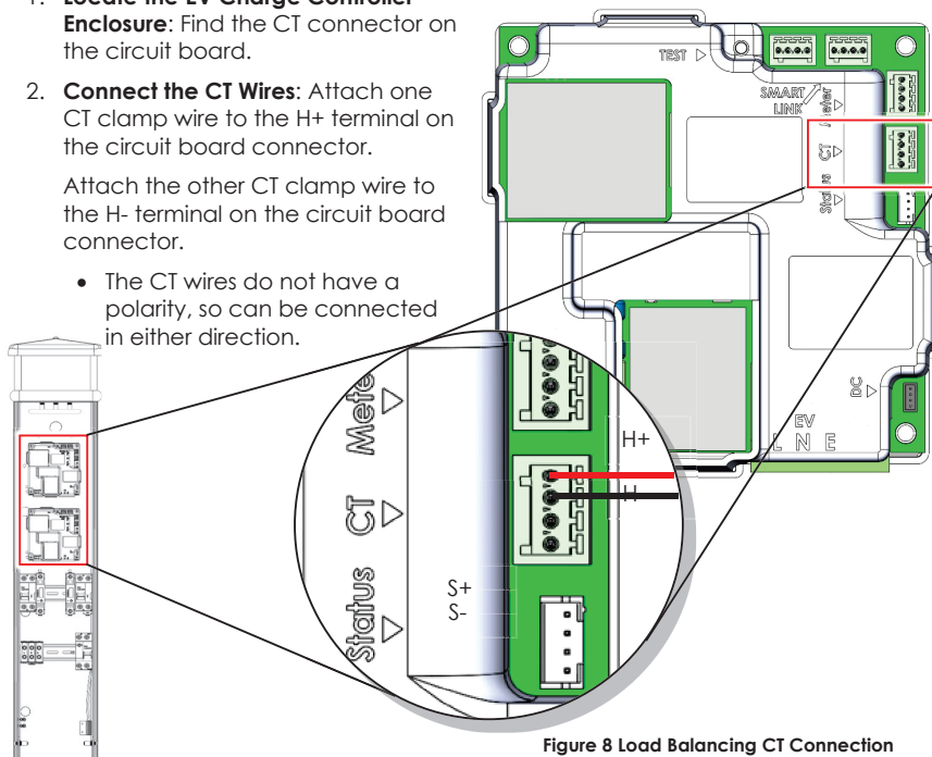
Figure 8 Load Balancing CT Connection
