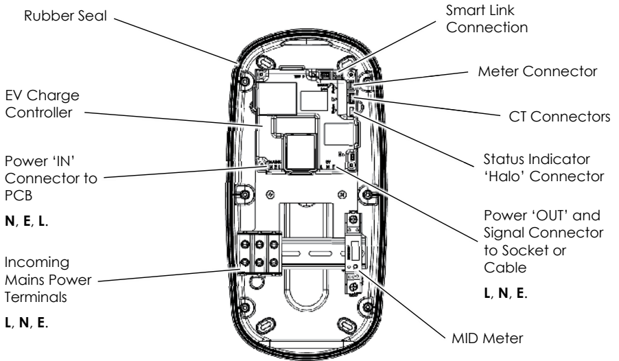
Figure 2 WallPod Rear Enclosure Components (For clarity, Wiring is not shown)
