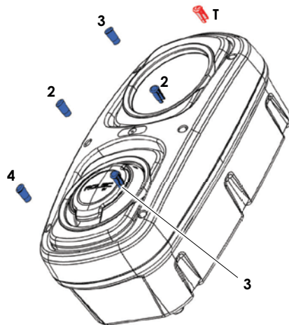
Figure 20 Anti-tamper Plug Locations
