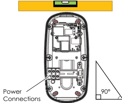
Figure 13 WallPod Alignment
