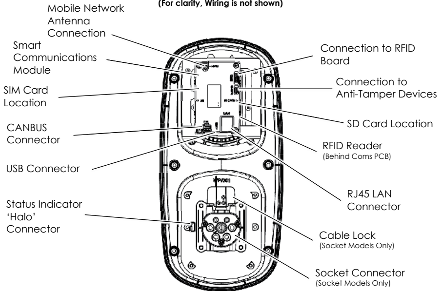
Figure 3 WallPod Front Enclosure Components (For clarity, Wiring is not shown)
