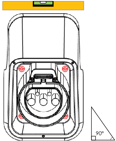
Figure 17 Mount the Plug Holster
