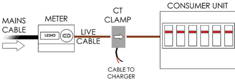
Figure 14 CT Clamp Positioning
