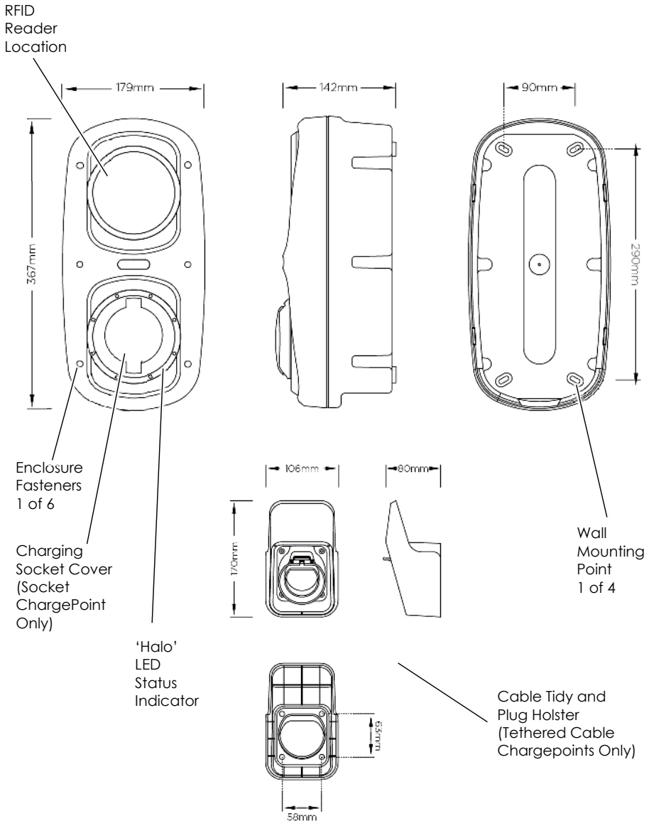
Figure 1 WallPod General Arrangement and Dimensions
