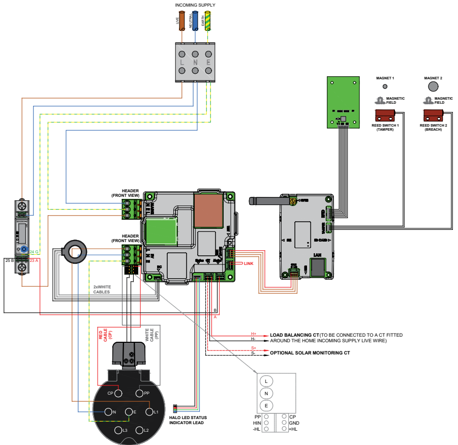
Figure 11 WallPod Intelligent EV Charging Unit – 1x up to 7.4kW Type 2 Socket
