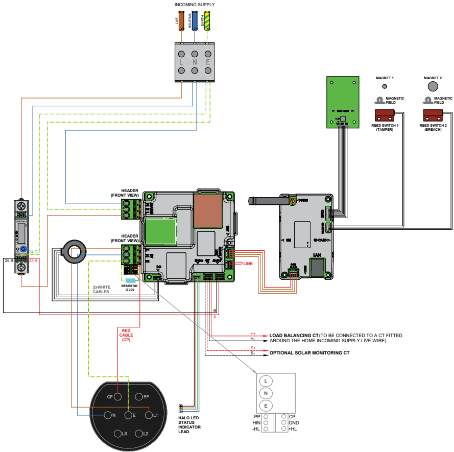
Figure 12 WallPod Intelligent EV Charging Unit – 1x up to 7.4kW Type 2 Tethered Cable
