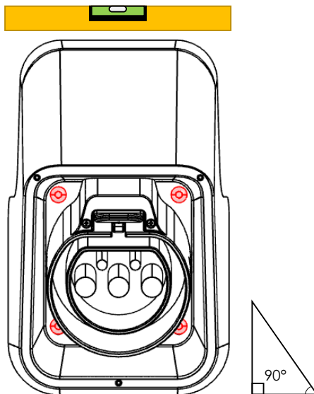
Figure 17 Mount the Plug Holster
