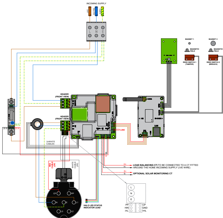
Figure 11 WallPod Intelligent EV Charging Unit – 1x up to 7.4kW Type 2 Socket
