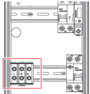
Figure 16 Incoming Mains Power Terminals (Single Phase Shown)
